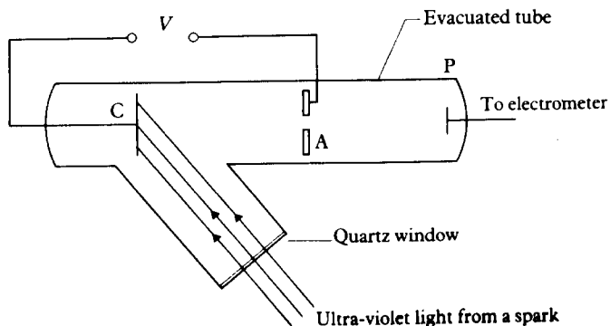
1.6 Lenard's apparatus for investigating the photoelectric effect.
